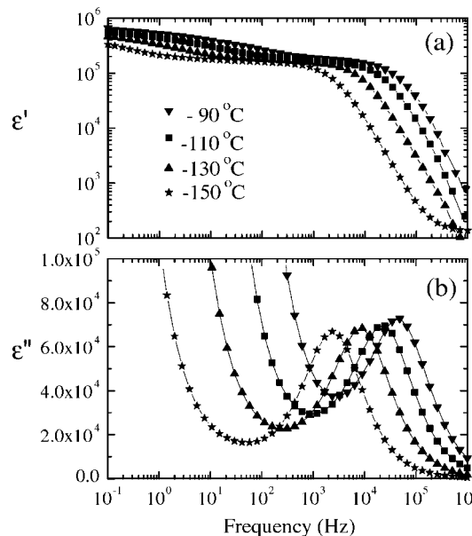
Figure 7. Frequency dependence of permittivity \epsilon^* in the sample made from the combustion method at several temperatures: (a) real part \epsilon' ; (b) imaginary part \epsilon'' .
