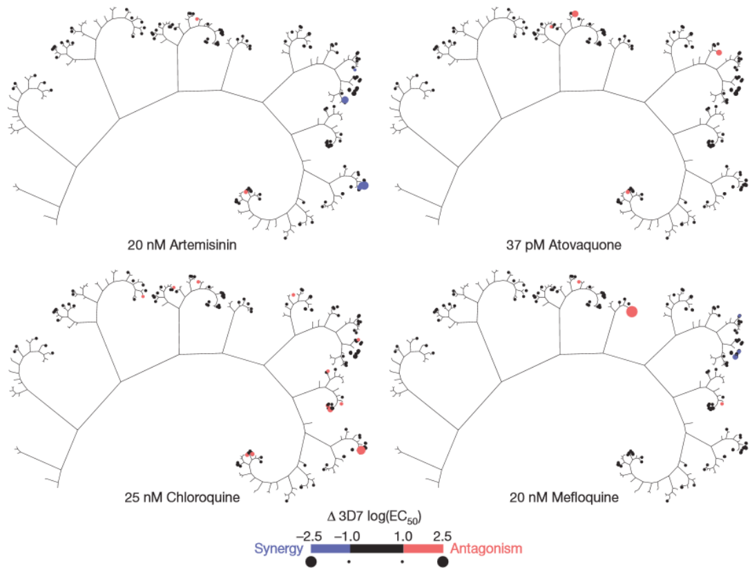
Figure 2 | Reduced representation of the network map showing synergistic activities with clinically relevant antimalarials. The size of the nodes reflects the magnitude of the logarithmic difference between EC^{50} in the presence and absence of EC^{10} of exemplar antimalarial drugs. Absolute differences less than one log unit were not considered significant. Synergistic and antagonistic compounds are uniformly colour-coded blue and red respectively. Highly synergistic compounds can be seen with artemisinin and mefloquine. Data are in Supplementary Information.
