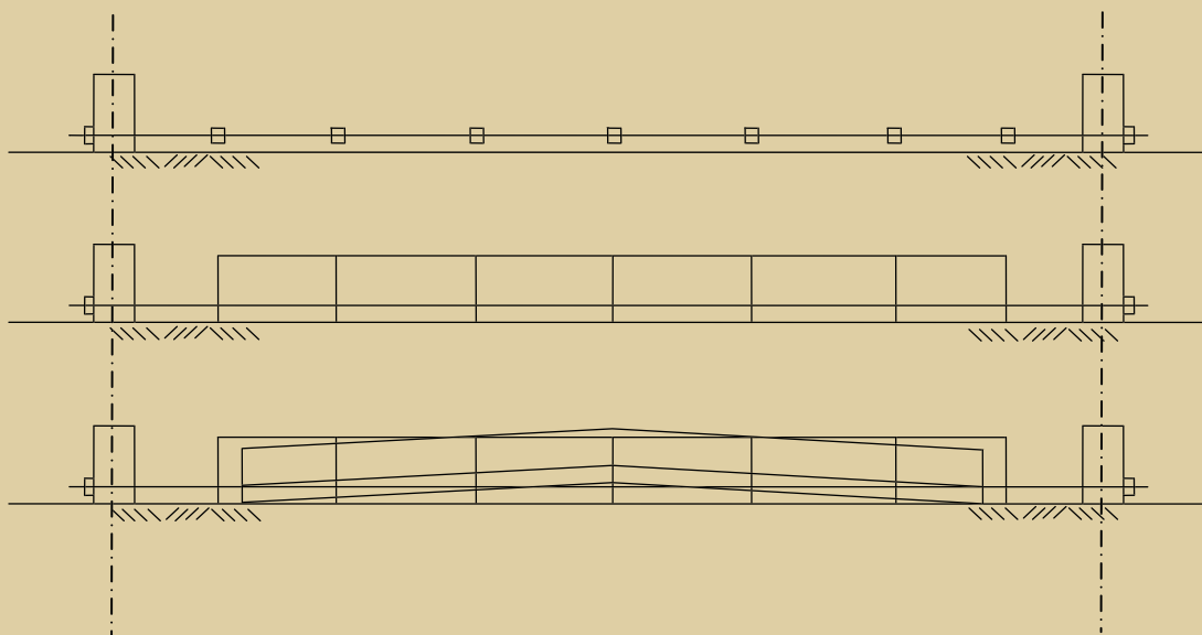
Figure 8. The fabrication sequence for pretensioning a curved precast concrete girder is the same as for straight girders. Note: The drawing is not to scale, and the camber is exaggerated.
