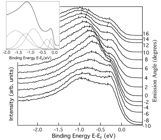
Figure 2. The photoemission spectra of \text{CoS}_2(001) for different emission angles from -10^\circ to +16^\circ , taken at a photon energy of 43 eV. The tick marks indicate the contributions to the spectra with strong surface weight i.e. conservation of two dimensionality of state (features that show little photon energy dependence). The inset shows a photoemission spectrum taken at 46 eV photon energy and with a larger accumulation of counts collected along the surface normal. For the inset some of the components of the photoemission spectra are indicated.
