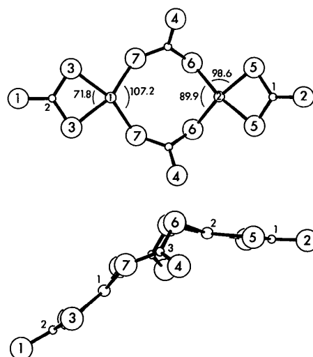
Fig. 2. Sketches of the Cu 2 (BO 3 ) 4 unit. Top: view along [100]. Angles in °. Bottom: view along direction orthogonal to mirror plane at y = \frac{1}{4} .
