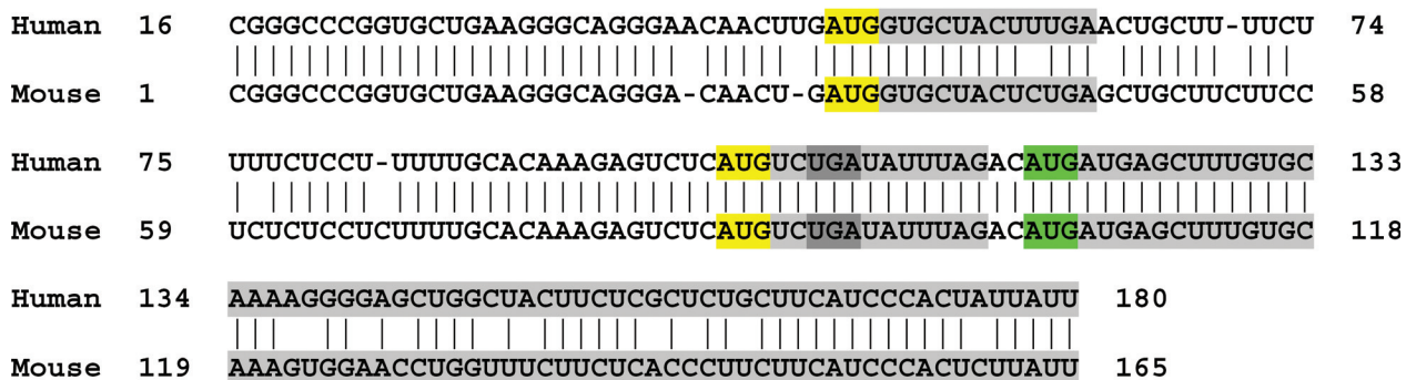
Figure 2. A mammalian 5'-UTR with conserved uAUGs and an in-frame stop codon. The alignment of the 5'UTRs of human and mouse \alpha 1 type III collagen proprotein (GI numbers: 15 149 480 and 33 859 525, respectively). uAUGs are colored yellow, the collagen starting codon is colored green, and the open reading frames are colored grey. The protein-coding region cannot be extended in the 5' direction because of the presence of a conserved in-frame UGA stop codon (dark gray).
