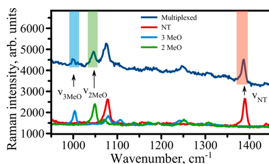
Figure 6. Proof-of-principle multiplex assay with three distinct Raman Reporter Molecules. Individual Raman spectra overlaid are shown in the bottom. The spectra correspond to RRM: 3 methoxybenzenethiol (3MeO—light blue), 2 methoxybenzenethiol (2MeO—green), and naphthalenethiol (NT—red). The dark blue spectrum above is the spectrum taken on a multiplexed assay where 3MeO, 2MeO, and NT are used as three distinct SERS labels for multiplexing. Spectra are shifted for visual clarity.
