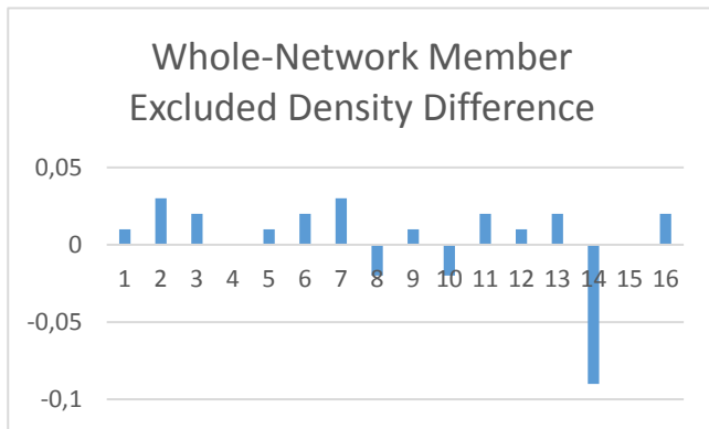
Figure 3. Whole-Network Member Excluded Density Difference.
