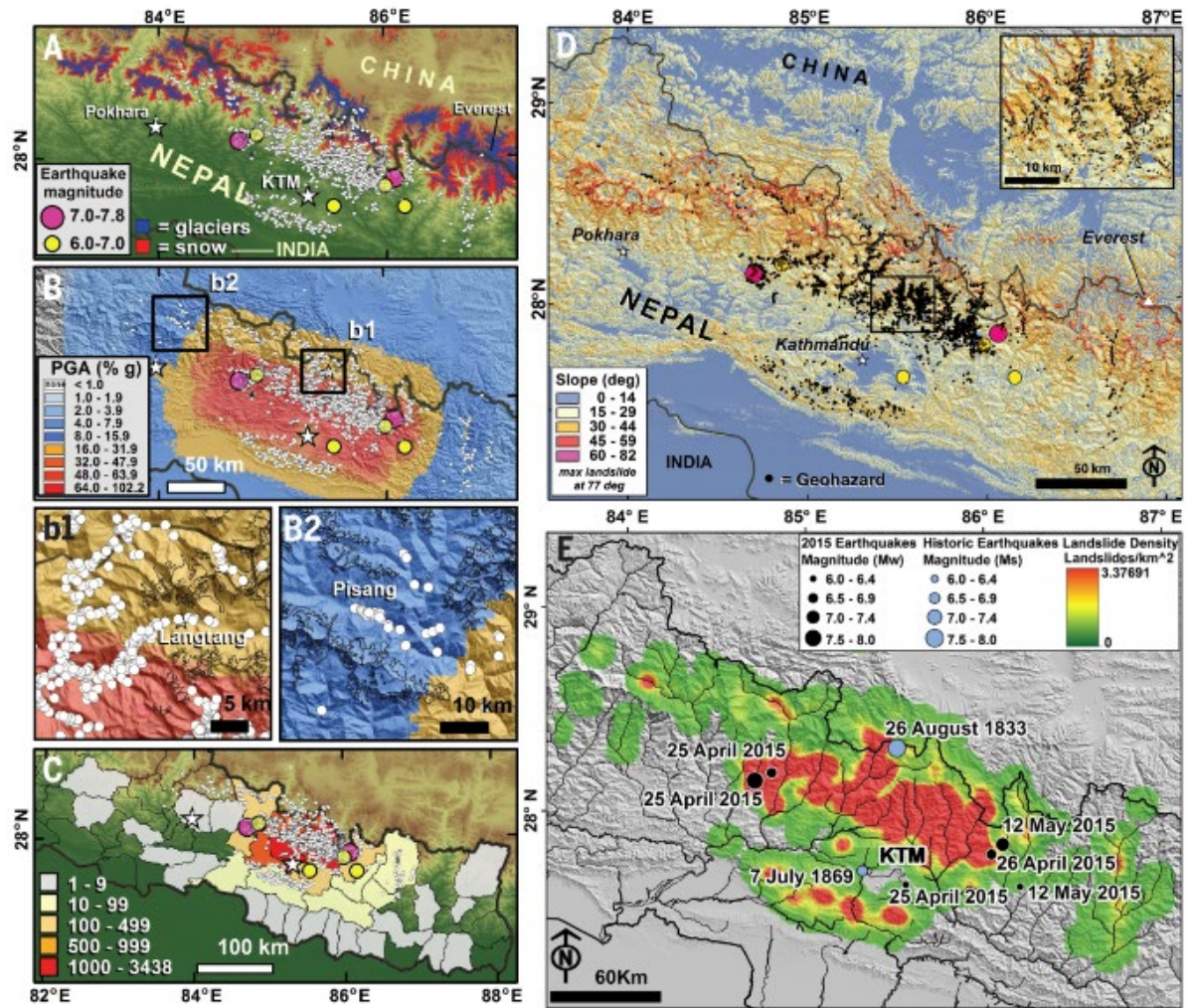
Fig. 1 Location of 4312 earthquake-related geo-hazards. (A) Distribution of glaciers (blue), late-season snowfields (red), landslides (white dots), and main shock and largest aftershock epi-centers. The base topography is from the SRTM 90-m gap-filled digital elevation model (33). Glacier extents are from the Randolph Glacier Inventory (RGI) (61). Snowfields were derived from pre-event Landsat-8 visible and near-infrared (VNIR) to short-wave infrared (SWIR) band ratios and topographic masks. (B) (Top) Landslides plotted with local peak ground accelerations induced by the main Gorkha shock or M>6 aftershocks. PGAs are from the USGS-National Earthquake Information Center ShakeMap (62). (Bottom) Boxes b1 and b2 are enlarged to show details near Langtang and Pisang. (C) Landslides plotted with reported deaths per Nepal district are from the Government of Nepal, Nepal Disaster Risk Reduction Project. (D) Hazard occurrences (black dots) on calculated slopes. (Inset) Detail of hazard-dense region. (E) Smoother area density (log scale) of earthquake-induced landslides determined by using a neighborhood 1/8^\circ by 1/8^\circ search window ( \sim 14 by 12 km) in relation to major ( M \geq 6 ) epicenters of historic earthquakes and the Gorkha quakes (62), Densities range between 0.01 and 3.37 landslides/km 2 . Higher landslide densities occur locally on
