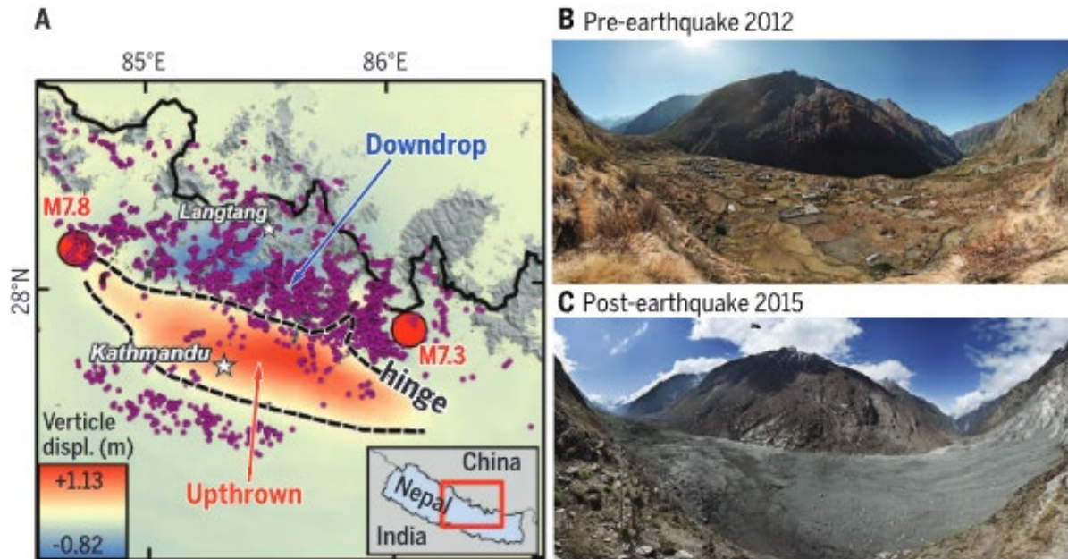
Landslide distribution and effects of a huge landslide. (A) Landslides (purple dots) are concentrated mostly north of the tectonic hinge-line. Also shown are the epicenters of the main shock and largest aftershock. Displacements are from the JAXA ALOS-2 ScanSAR interferogram (21 Feb and 2 May 2015 acquisitions). (B and C) Before-and-after photographs obtained by D. Breashears in Langtang Valley showing complete destruction of a large part of Langtang village by a huge landslide.
