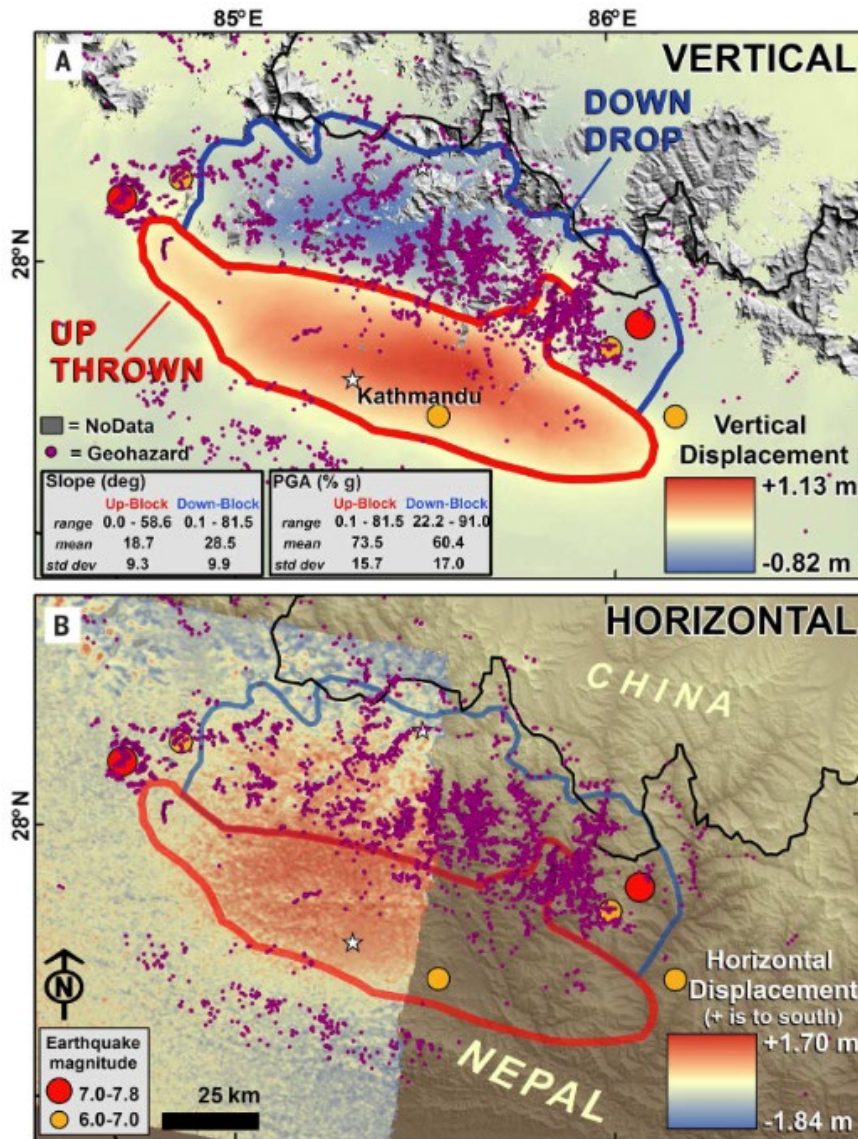
Fig. 3. Landslide distribution relative to the Earth surface deformation field. (A) 4312 landslides (purple dots) are concentrated mostly north of the hinge line between the downdropped block and uplifted block. Also shown are the epicenters of the main shock and five largest aftershocks. Vertical displacements are from the JAXA ALOS-2 ScanSAR interferogram (21 Feb and 2 May 2015 scenes), which represent almost entirely vertical motion. ALOS-2 interferometry of the Gorkha earthquake and largest aftershock was recently described by Lindsey et al. (3). (B) Horizontal motion map based on azimuth shift measurements of the RADARSAT-2 XFacquisitions of 5 April and 29 April 2015. Scale shows motion excluding outliers outside the mean \pm 3s . Values are positive for SSW azimuths >100 degrees relative to east ( >S10W ). Hence, both the upthrown and downdropped blocks shifted southward. The areal coverage for the RADARSAT-2 scene is not identical to that of ALOS-2; areas on the eastern side of the scene have no data.
