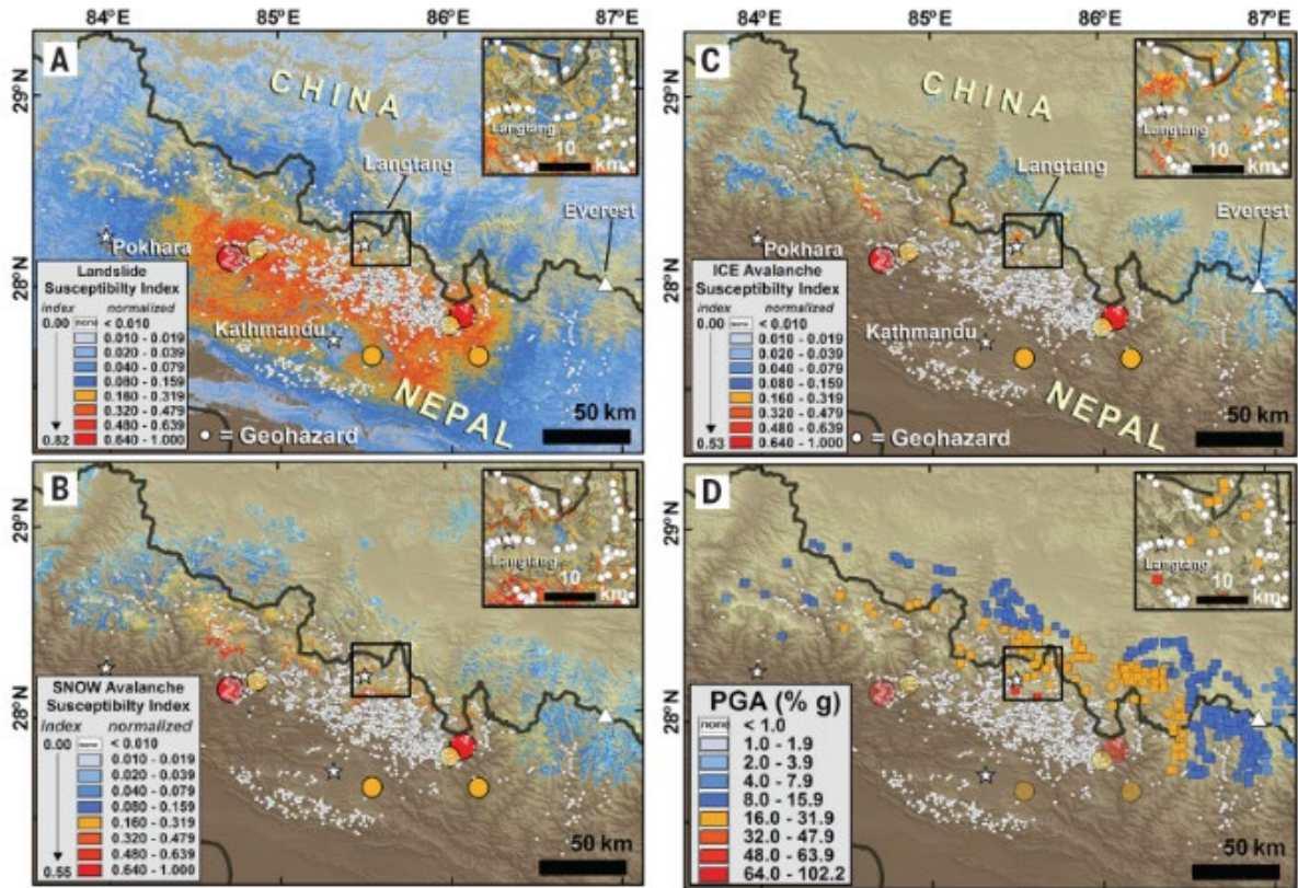
Fig. 2. Debris landslide susceptibility with mapped hazards. (A) Susceptibility in units of acceleration divided by g ( 9.81 \text{ m s}^{-2} ). (B) Snow avalanche susceptibility with mapped hazards. Susceptibility is in g . (C) Ice avalanche susceptibility with mapped hazards. Susceptibility is in g . (D) Maximum PGA experienced by 491 glacier lakes. Mapped hazards are shown as white dots. Maximum PGA for glacier lakes was 0.57g . (Insets) Detail in Langtang Valley.
