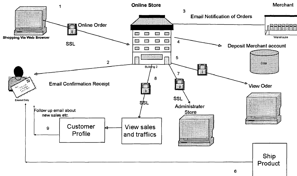
Figure2.1 e-commerce process diagram
